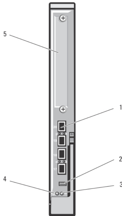
Figure 23. Commutateur Dell PowerConnect-KR 8024-k
